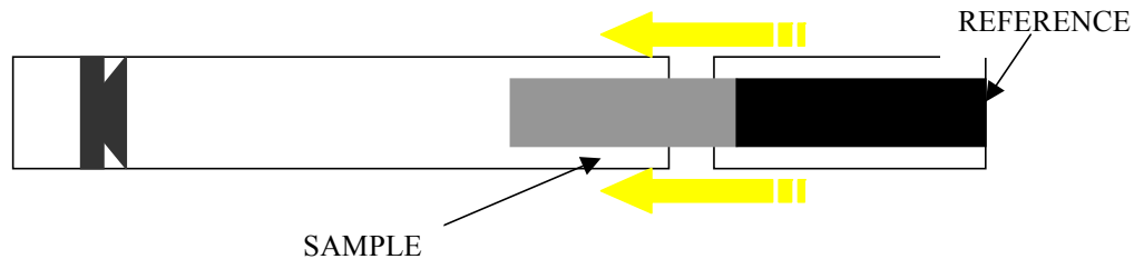
Figure 24 UNH impedance tube with reference backing material
